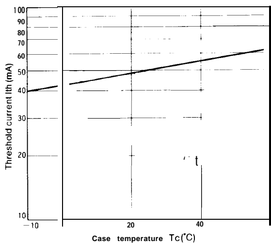
Fig. 71-3 Threshold Current vs. Temperature
