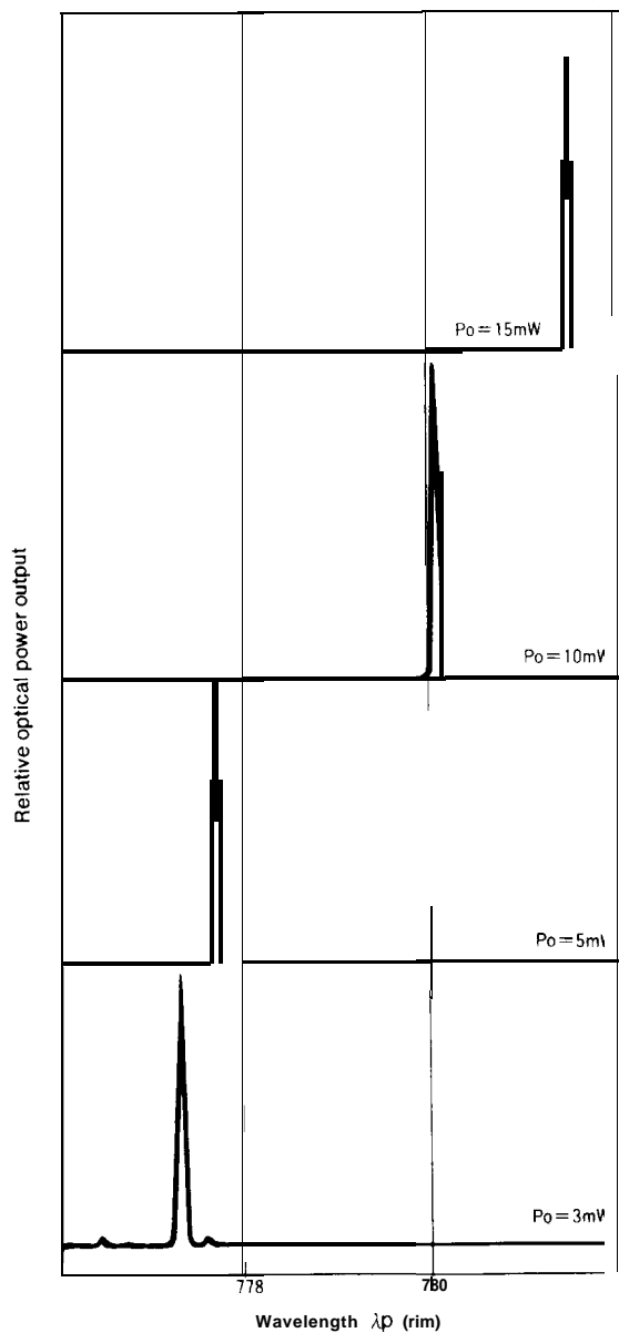
Fig. 71-5 Optical Power Output Dependence of Wavelength
