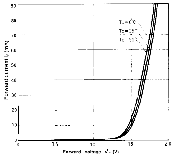
Fig. 71-1 Forward Current vs. Forward Voltage
