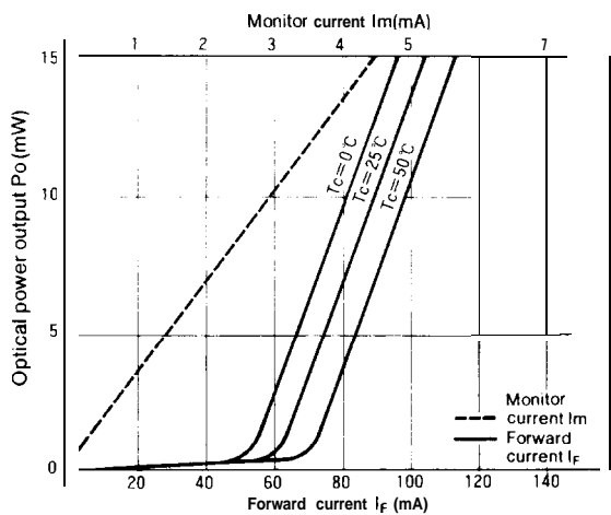
Fig. 71-2 Optical Power Output vs. Forward Current and Monitor Current
